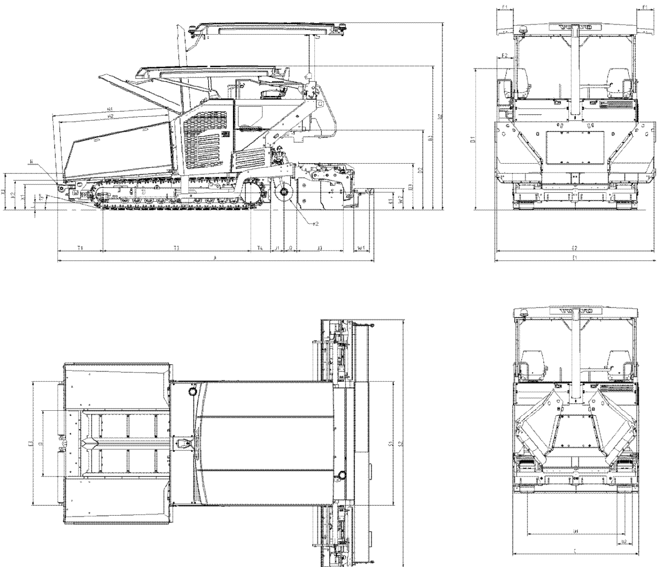
Figure 1 Dimensions, drawing
