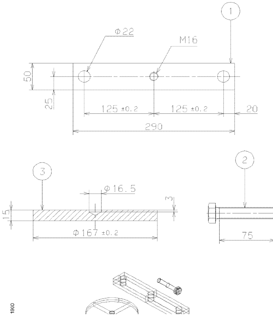
Figure 1 Press tool
