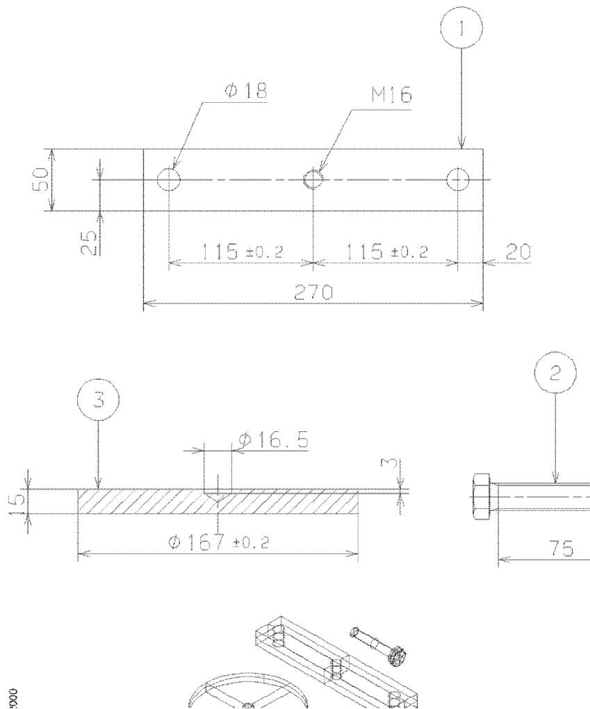
Figure 1 Press tool
