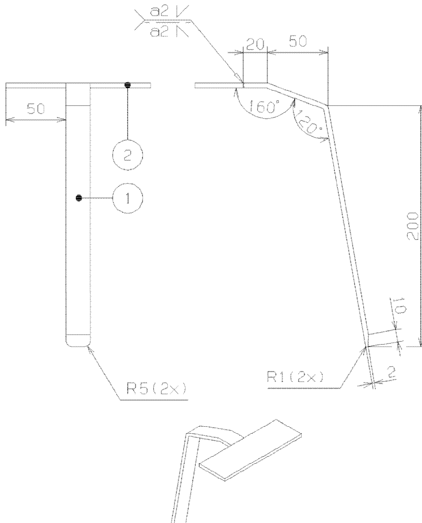
Figure 1 Assembly tool
