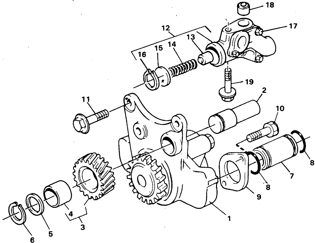
Volvo Construction Equipment FF 108
