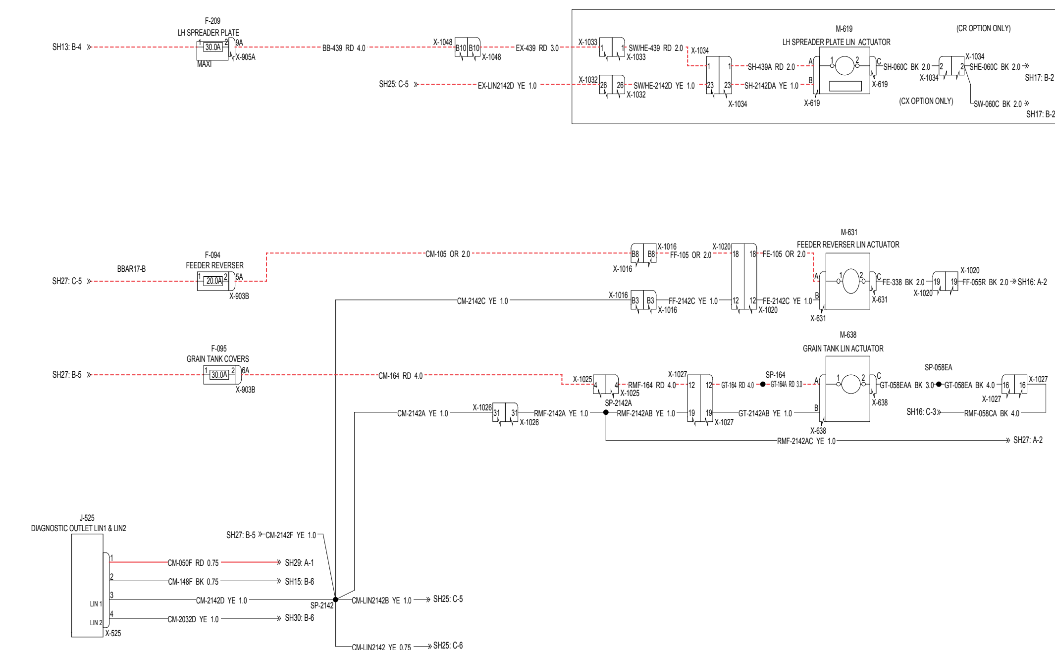
SHEET 28 - SPREADER PLATE, FEEDER REV & GRAIN TANK
