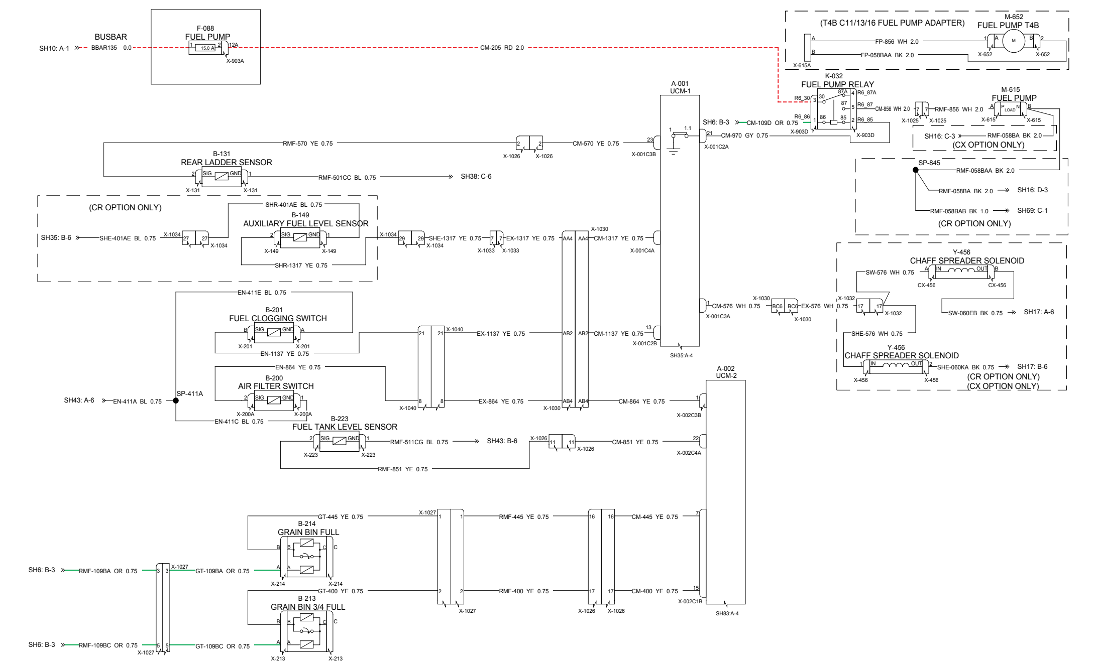
SHEET 45 - UCM1 AND UCM2 - GRAIN BIN/FUEL TANK
