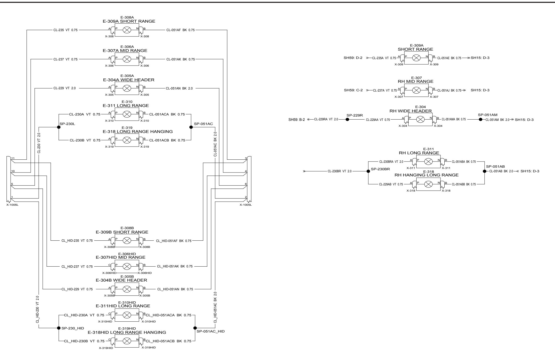
SHEET 48 - H-BRIDGE 1 AND 3
