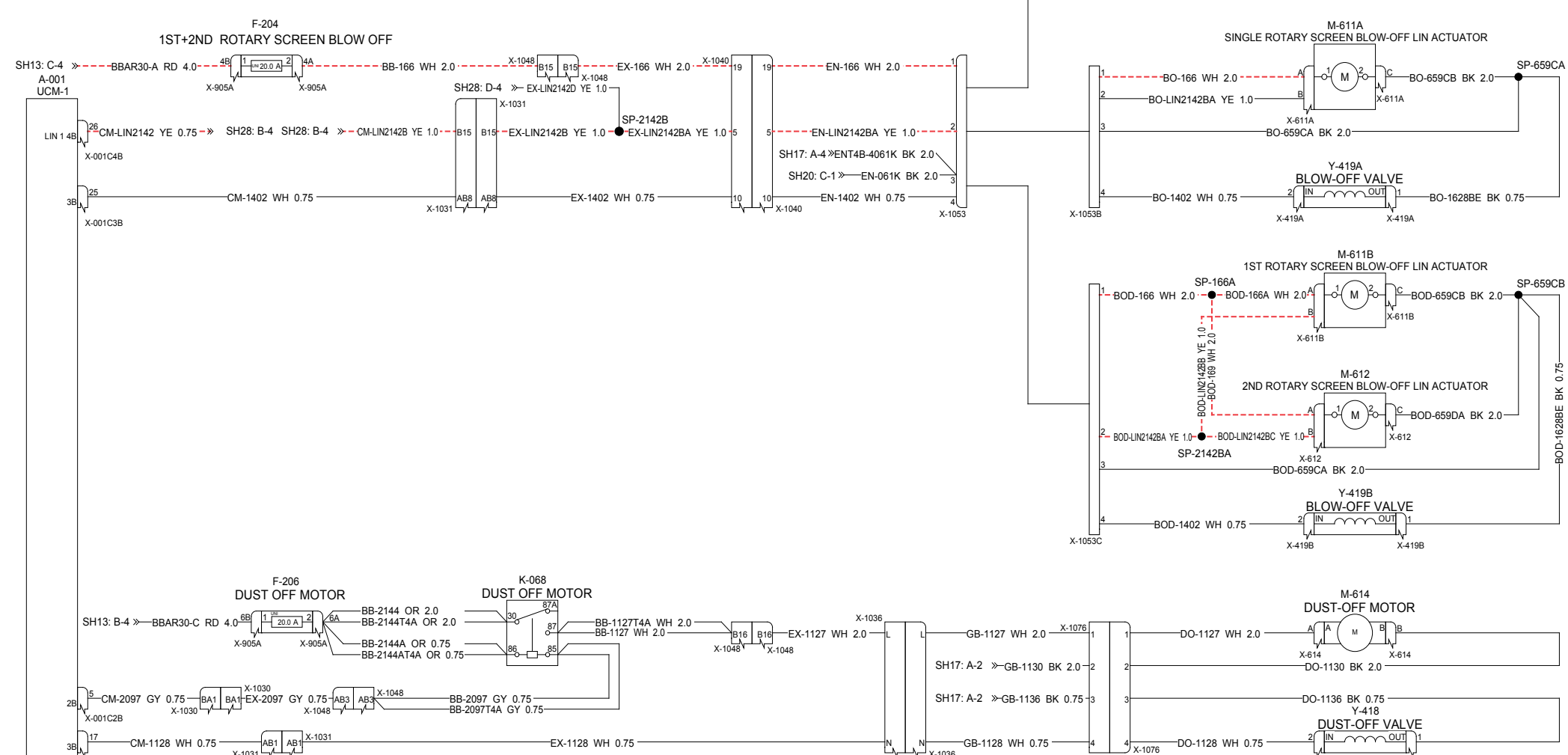
SHEET 25 - ENGINE: ROTARY BRUSH/BLOW/DUST-OFF
