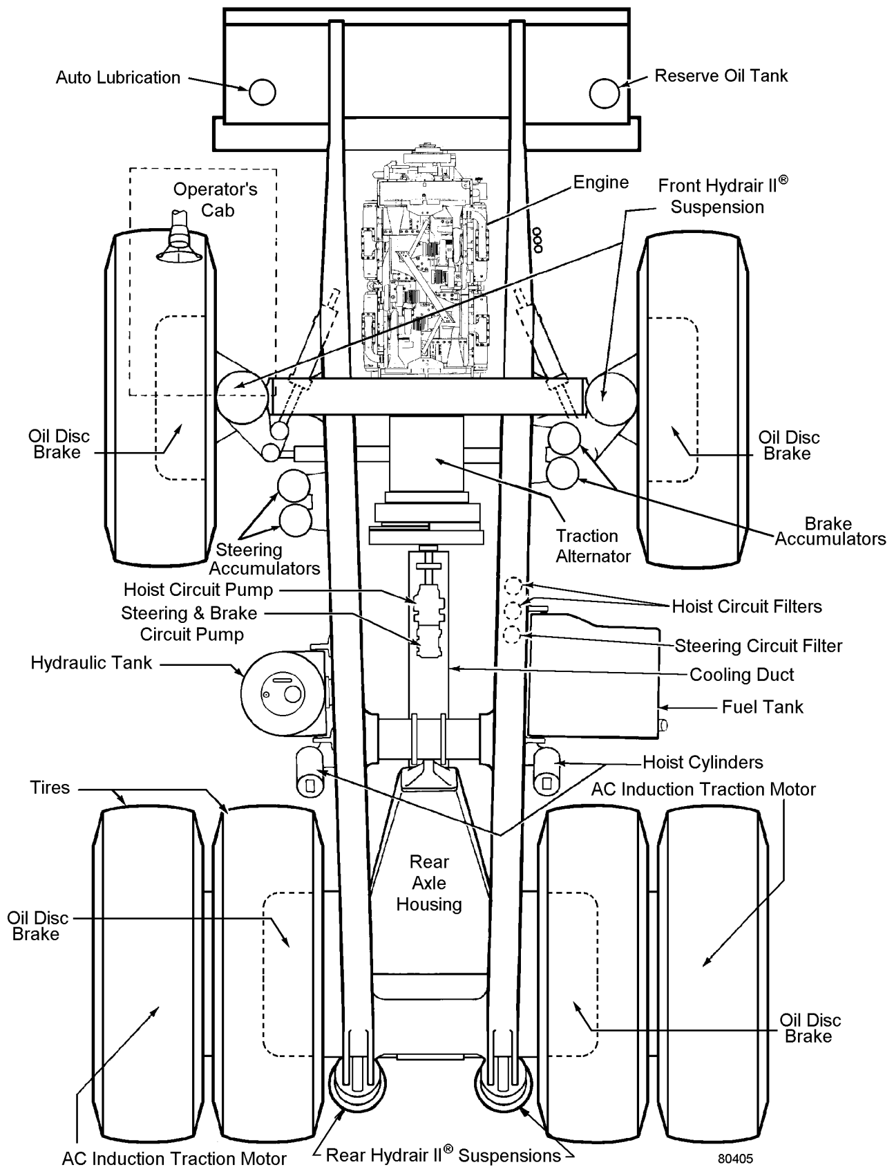
960E-1K MAJOR COMPONENTS
