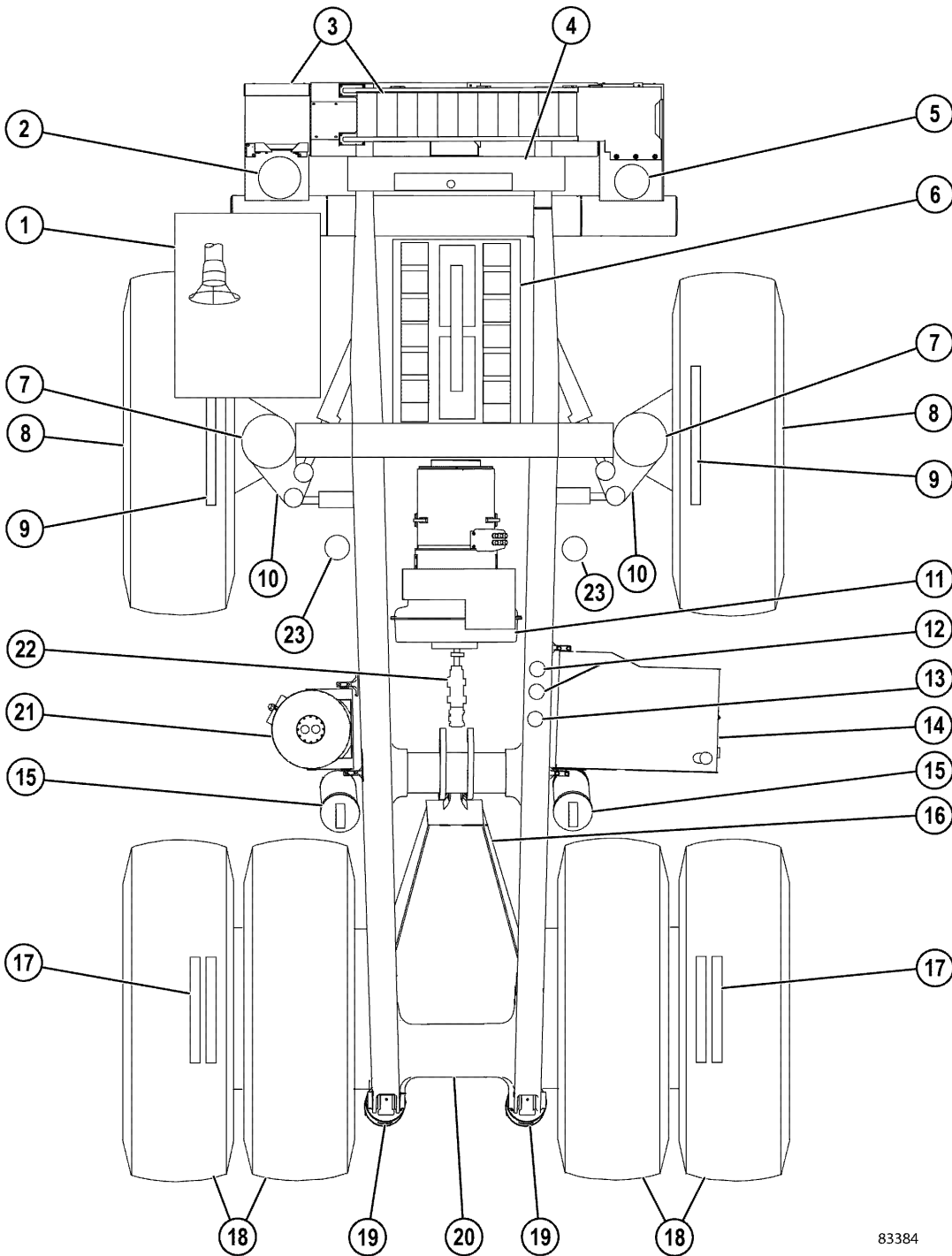
FIGURE 2-1. TRUCK COMPONENTS
