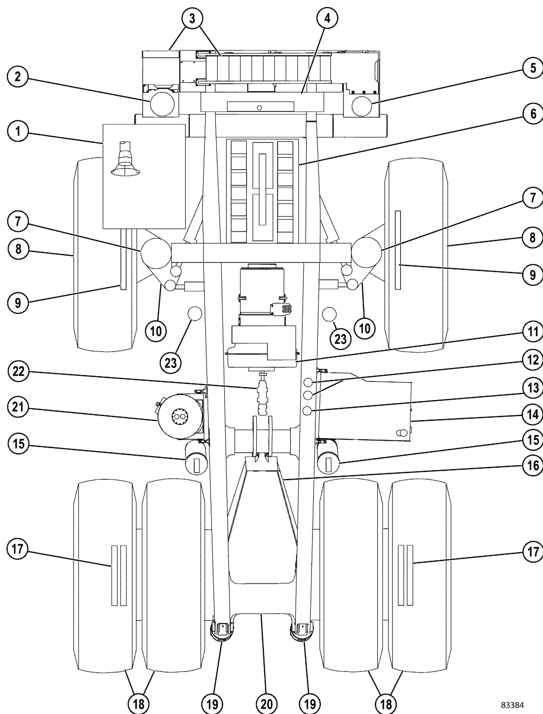
FIGURE 2-1. TRUCK COMPONENTS
