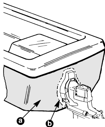
a - Antifouling Paint b - MINIMUM 1 inch (26 mm) UNPAINTED Area
